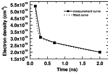
FIG. 4. The decay of the electron density in the plasma channel versus time.
